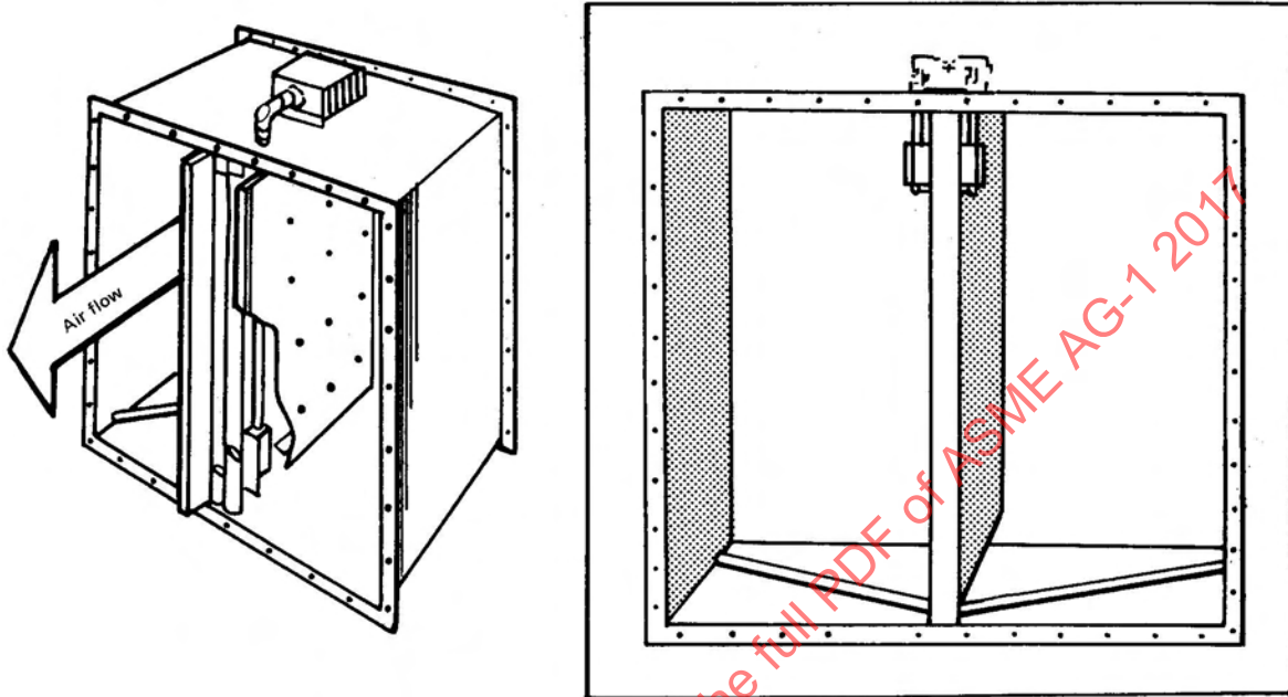
Wing Blade Damper
