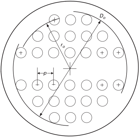
(a) Tubesheet Layout
