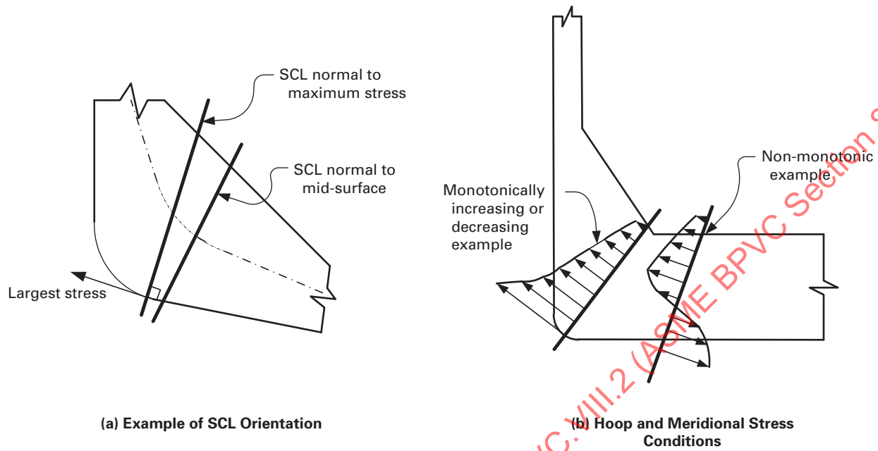
Figure 5-A.3 Stress Classification Line Orientation and Validity Guidelines
