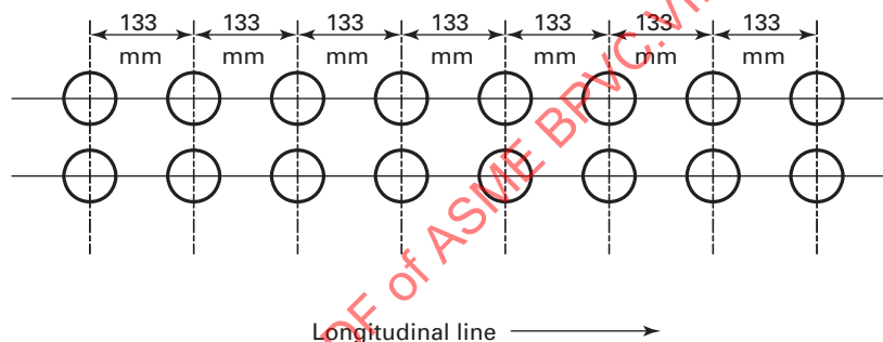
Figure 4.10.1 Example of Tube Spacing With the Pitch of Holes Equal in Every Row
