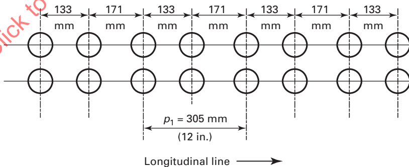
Figure 4.10.2 Example of Tube Spacing With the Pitch of Holes Unequal in Every Second Row
