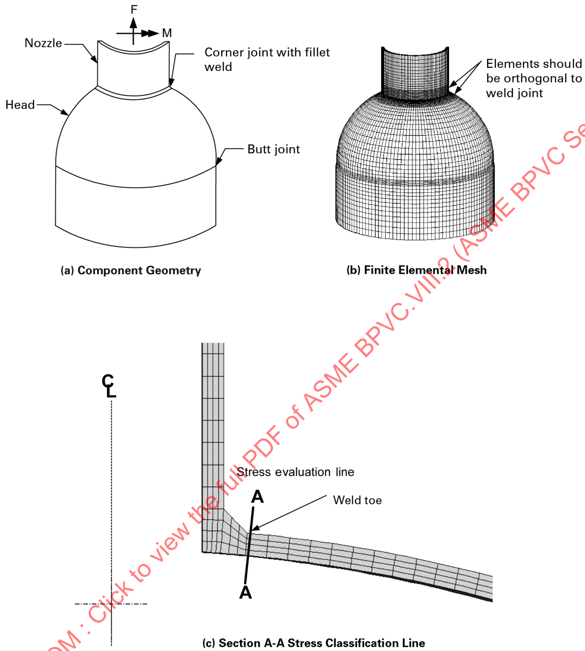
Figure 5-A.5 Continuum Finite Element Model Stress Classification Line for the Structural Stress Method
