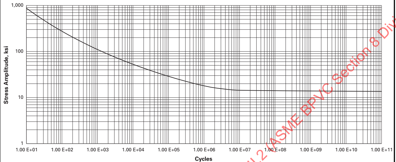
Figure 3-F.3 Fatigue Curve for Series 3XX High Alloy Steels, Nickel–Chromium–Iron Alloy, Nickel–Iron–Chromium Alloy, and Nickel–Copper Alloy for Temperatures Not Exceeding 800°F
