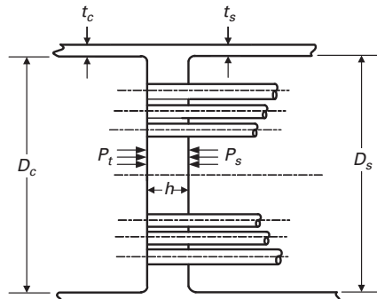
(a) Configuration a: Tubesheet Integral With Shell and Channel
