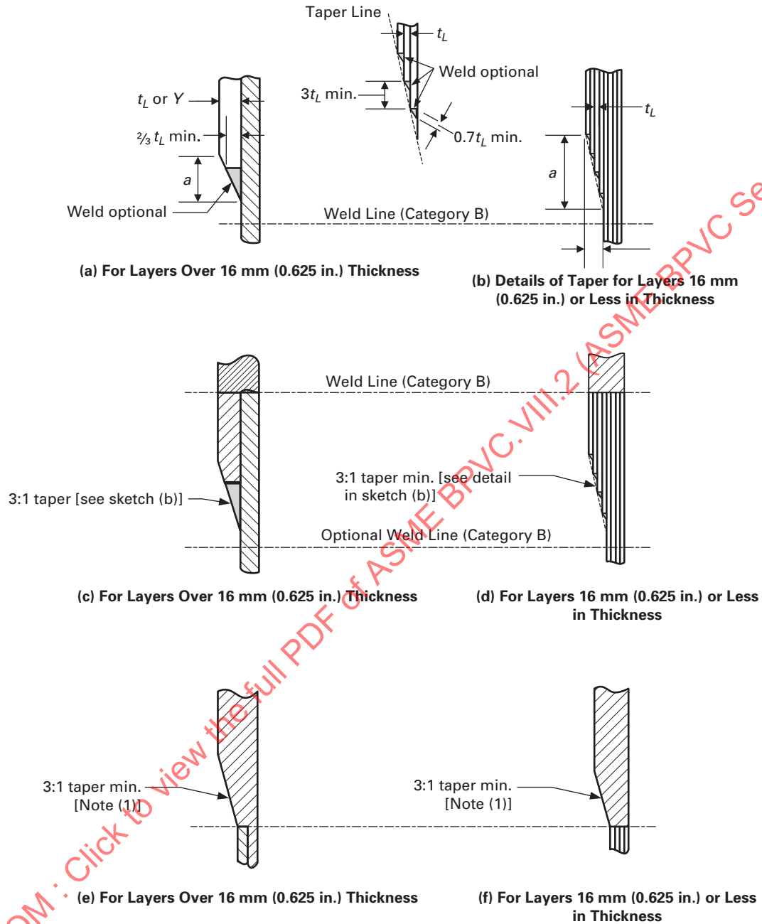
Figure 4.13.3 Transitions of Layered Shell Sections
