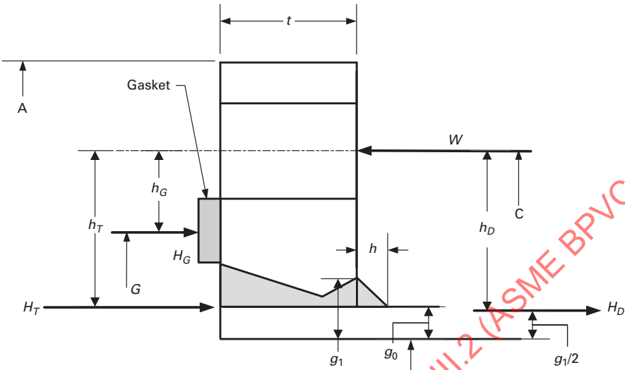
Figure 4.16.1 Integral Type Flanges
