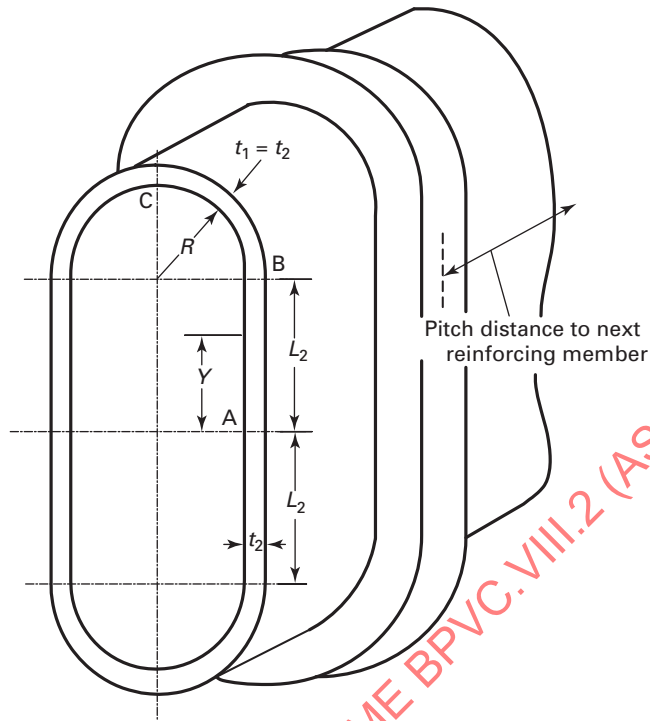
Figure 4.12.11 Type 10 Noncircular Vessels (Reinforced Obround Cross Section)
