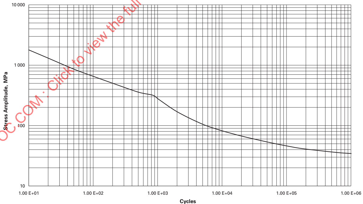
Figure 3-F.6M Fatigue Curve for Wrought 70–30 Copper–Nickel for Temperatures Not Exceeding 371°C — \sigma_{ys} = 310 MPa
