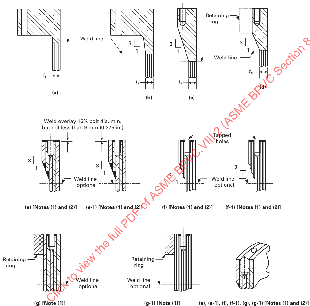
Figure 4.13.7 Some Acceptable Flanges for Layered Shells
