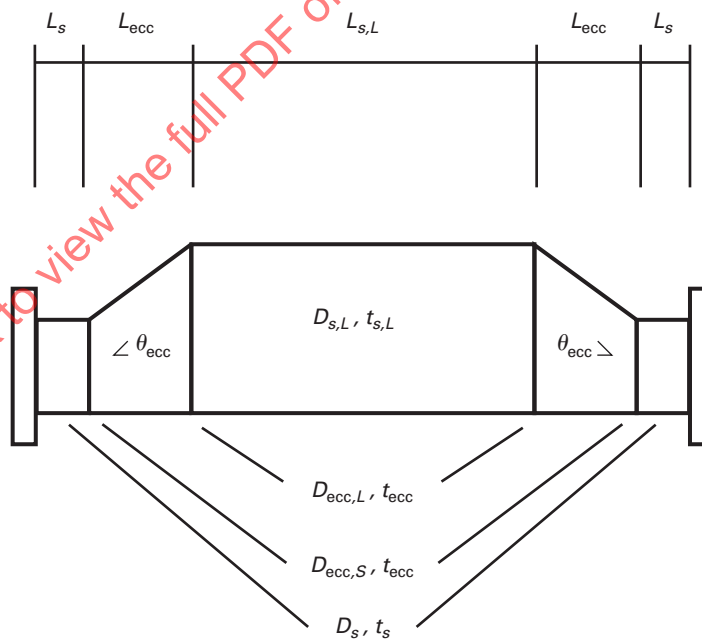
Figure 4.18.17 Kettle Shell
