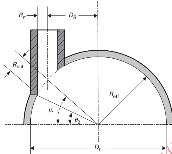
(a) Spherical Shell or Hemispherical Head
