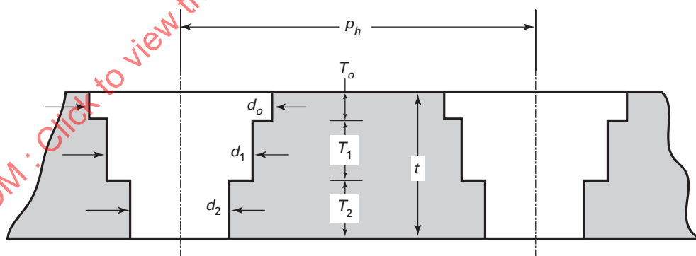
Figure 4.12.14 Multi-Diameter Holes
