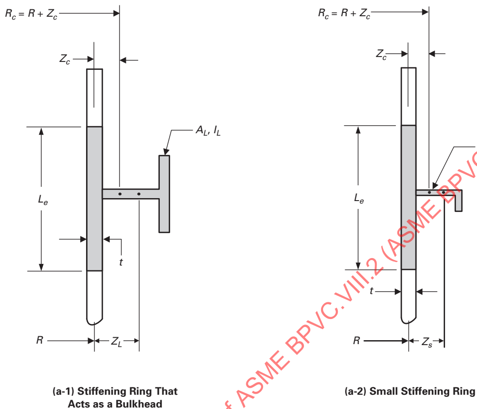
Figure 4.4.3 Stiffener Ring Parameters
