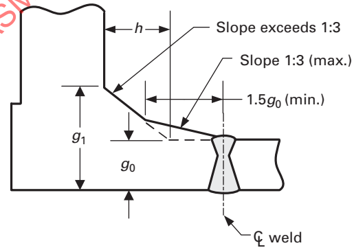
(c) Hub Type 3
