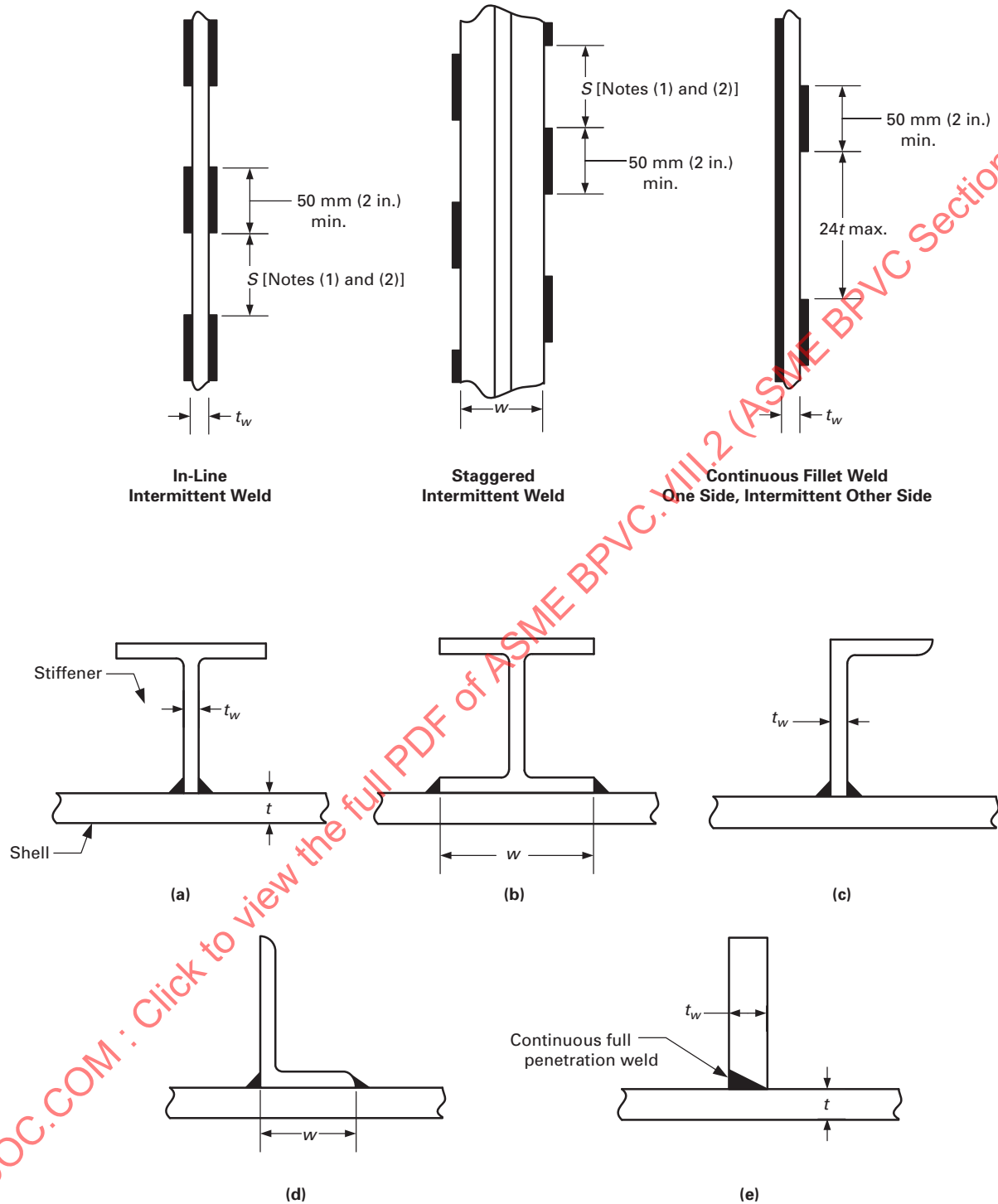
Figure 4.2.3 Some Acceptable Methods of Attaching Stiffening Rings
