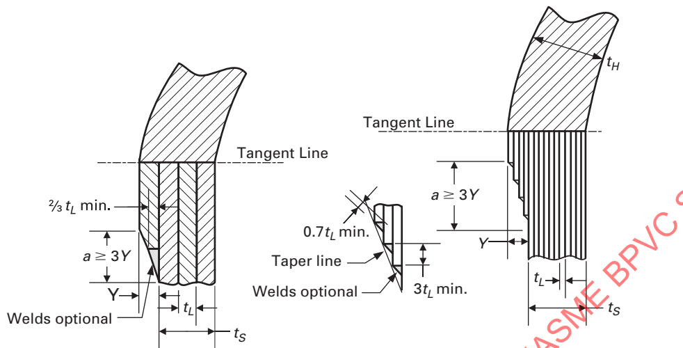
Figure 4.13.5 Some Acceptable Solid Head Attachments to Layered Shell Sections (Cont'd)
