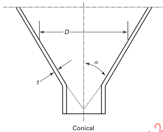
Figure 4.3.1 Conical Shell
