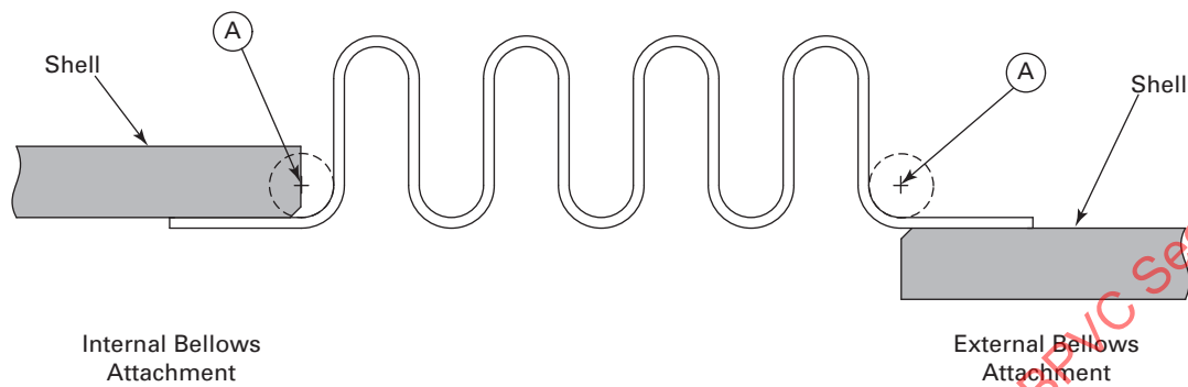
Figure 4.19.2 Starting Points for the Measurement of the Length of Shell on Each Side of Bellows
