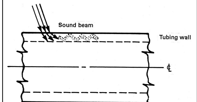
Figure KE-242.1 Axial Propagation of Sound in Tube Wall
