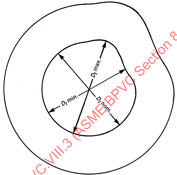
Figure KF-131 Examples of Differences Between Maximum and Minimum Diameters in Cylindrical Shells
