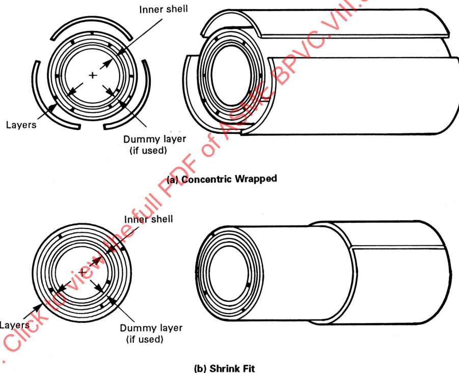
Figure KD-830.1 Acceptable Layered Shell Types
