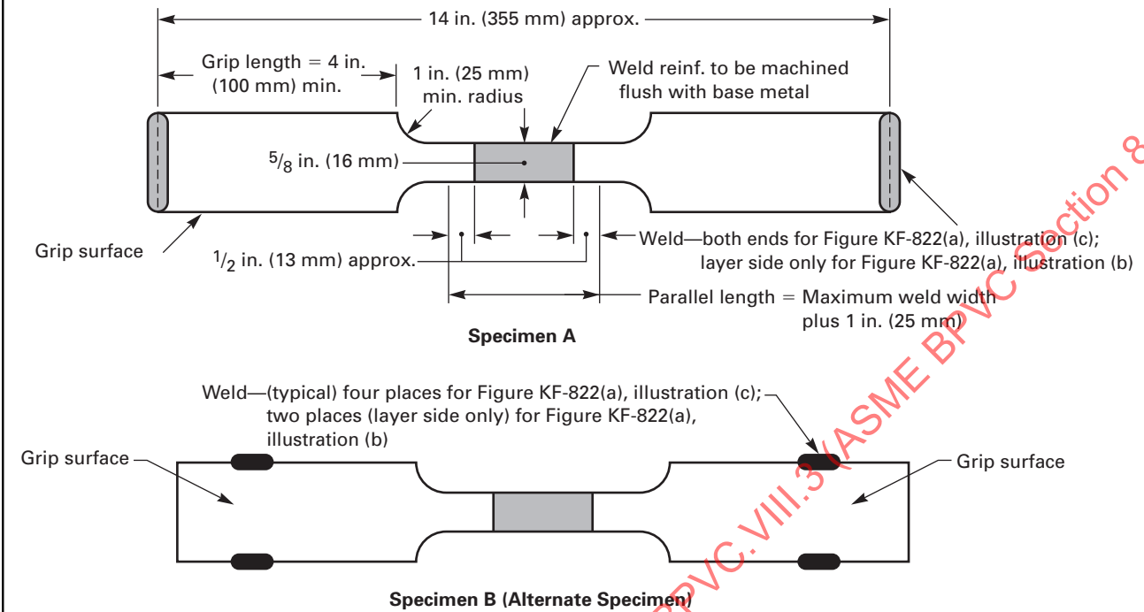
Figure KF-822(b) Test Specimens for Weld Procedure Qualification
