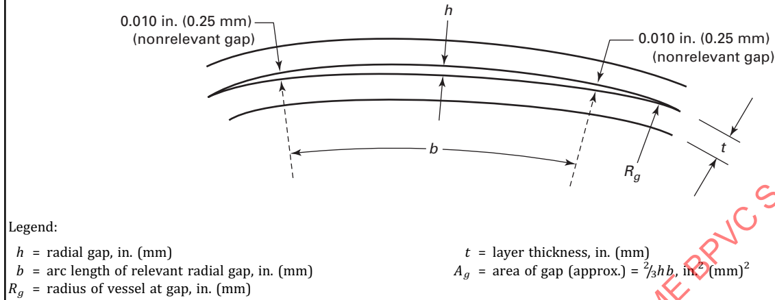
Figure KF-826 Gap Area Between Layers
