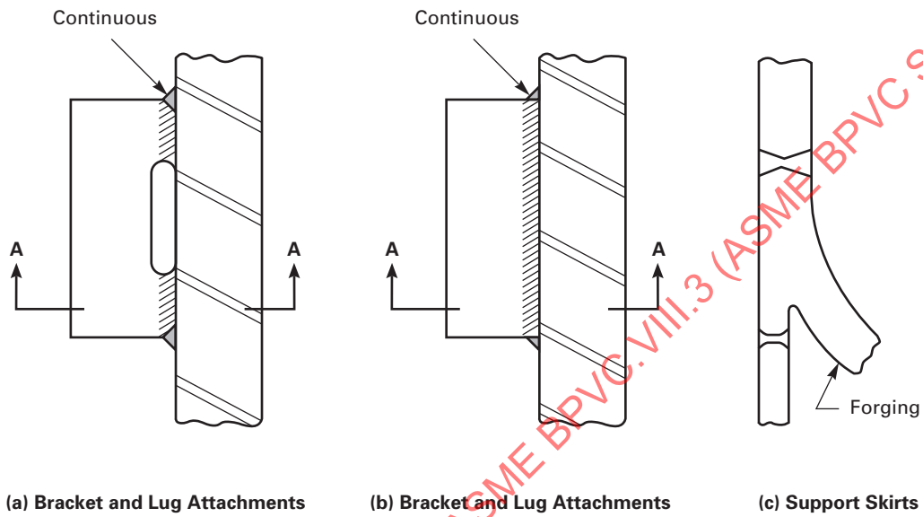
Figure KD-700 Some Illustrative Weld Attachment Details
