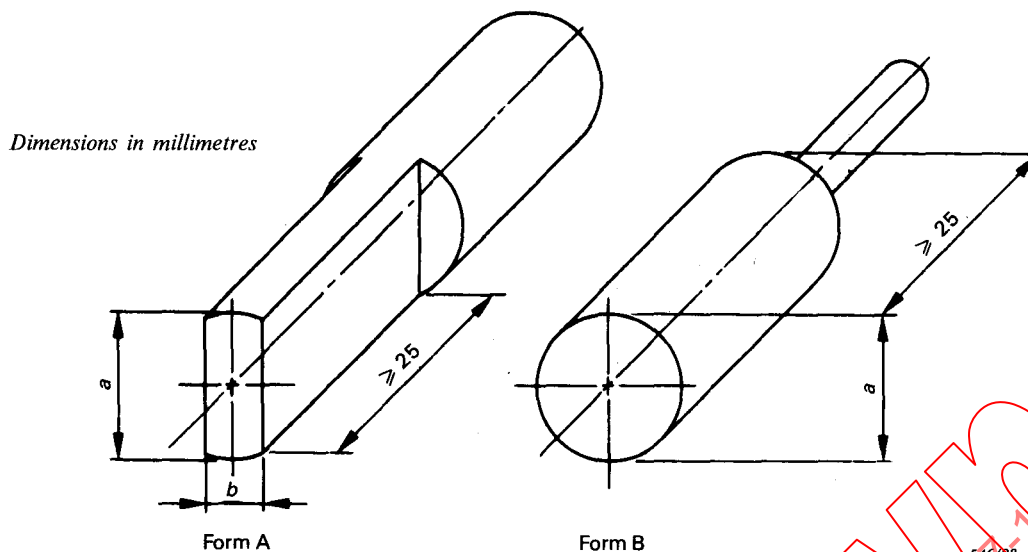
FIG. 2. — Gauges of form A and form B.
