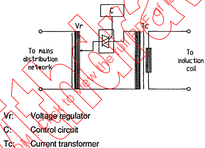
Figure 2 - Schematic circuit of the test generator for power frequency magnetic field.
