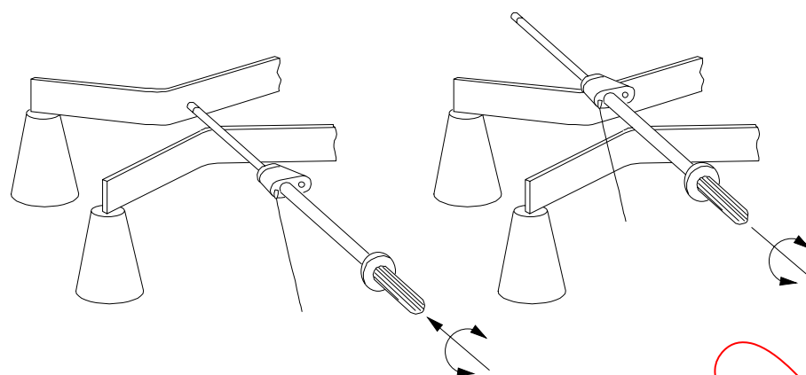
Figure 9 – Bridging protection, test run 2
