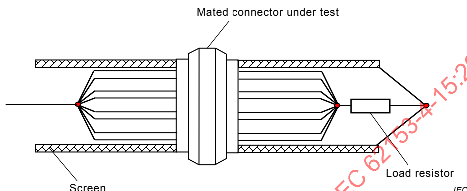
Figure 4 – Preparation of balanced or multipin connectors for transfer impedance and screening attenuation
