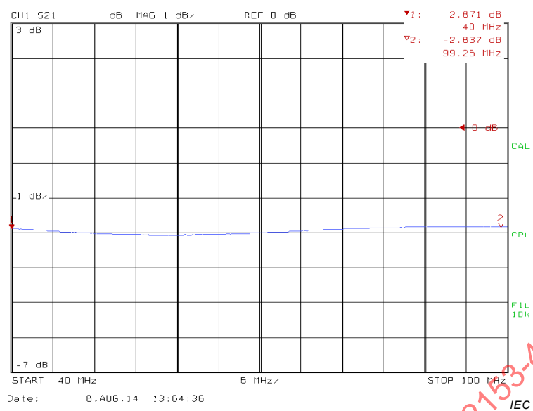
Figure E.2 – Measurement with ZVRE of S_{21} of a 3dB attenuator
