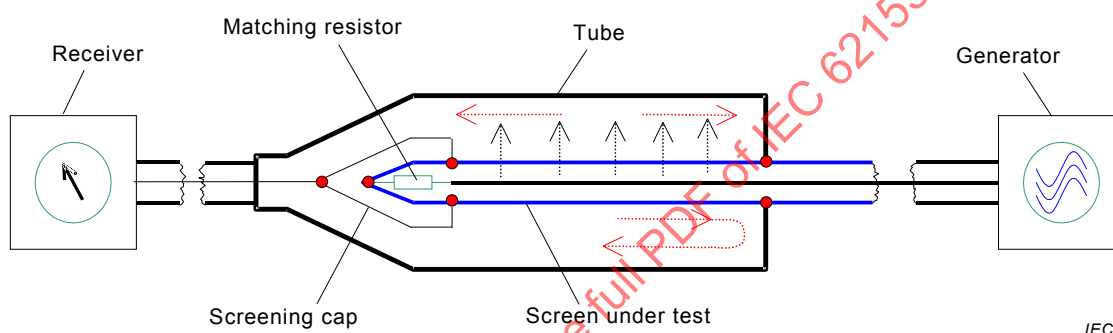
Figure A.1 – Principle test set-up to measure transfer impedance and screening attenuation
