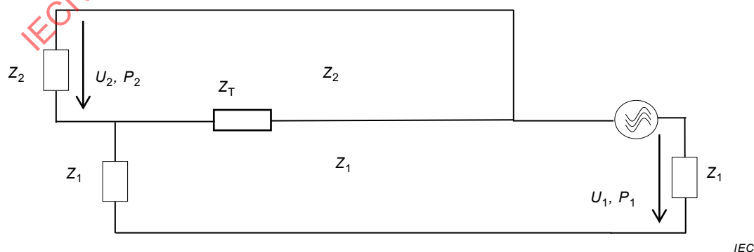
Figure A.2 – Equivalent circuit of the principle test set-up in Figure A.1
