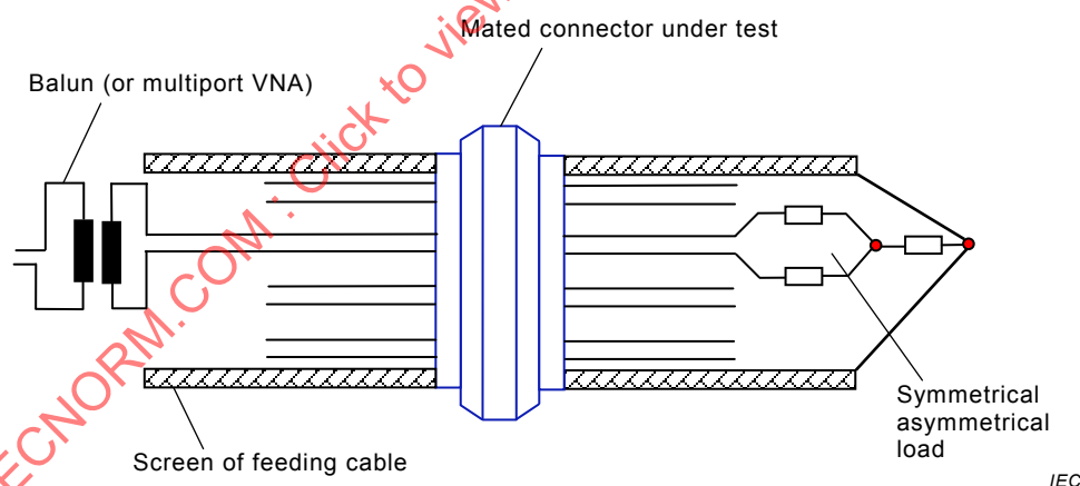
Figure 5 – Preparation of balanced or multipin connectors for coupling attenuation measurement
