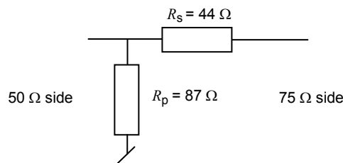
Figure B.3 – Coaxial impedance matching adapters (50 \Omega to 75 \Omega )
