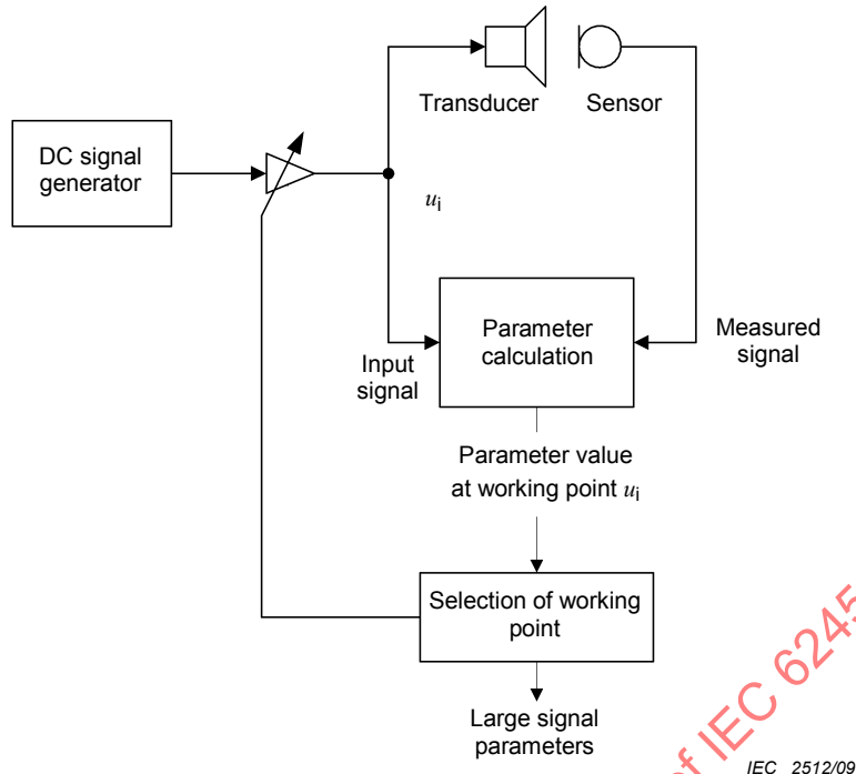
Figure 2 –Static and quasi-static measurement setup
