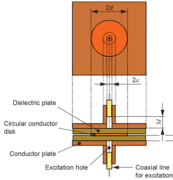
Figure 1 – Structure of a circular disk resonator
