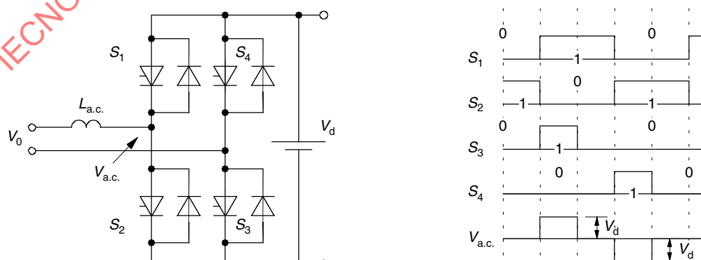
Figure 17 – Single-phase self-commutated rectifier (full bridge type)
