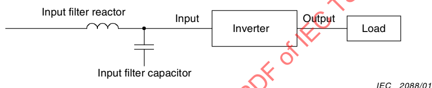
Figure 44 – Basic circuit configuration of a voltage-stiff inverter
