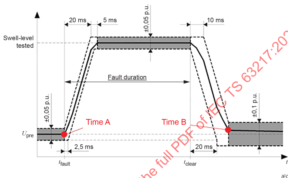
Figure 7 – Tolerance of voltage swell
