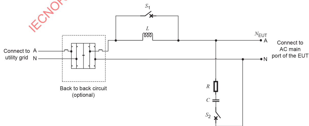
Figure 3 – RLC-series emulator for single-phase EUT
