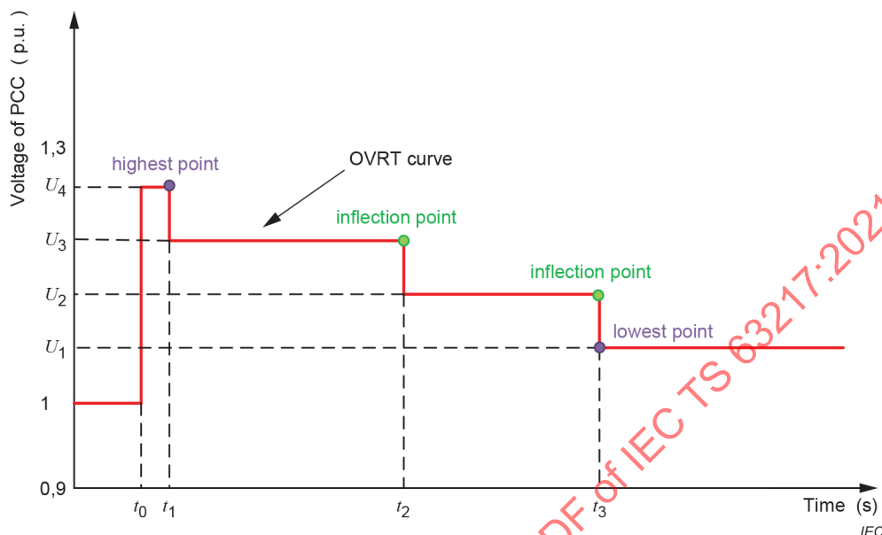
Figure 6 – OVRT curve example
