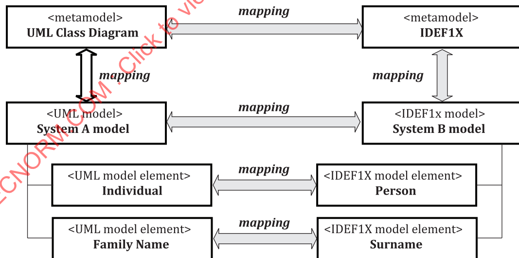
Figure B.1 — Registration of models and metamodels
