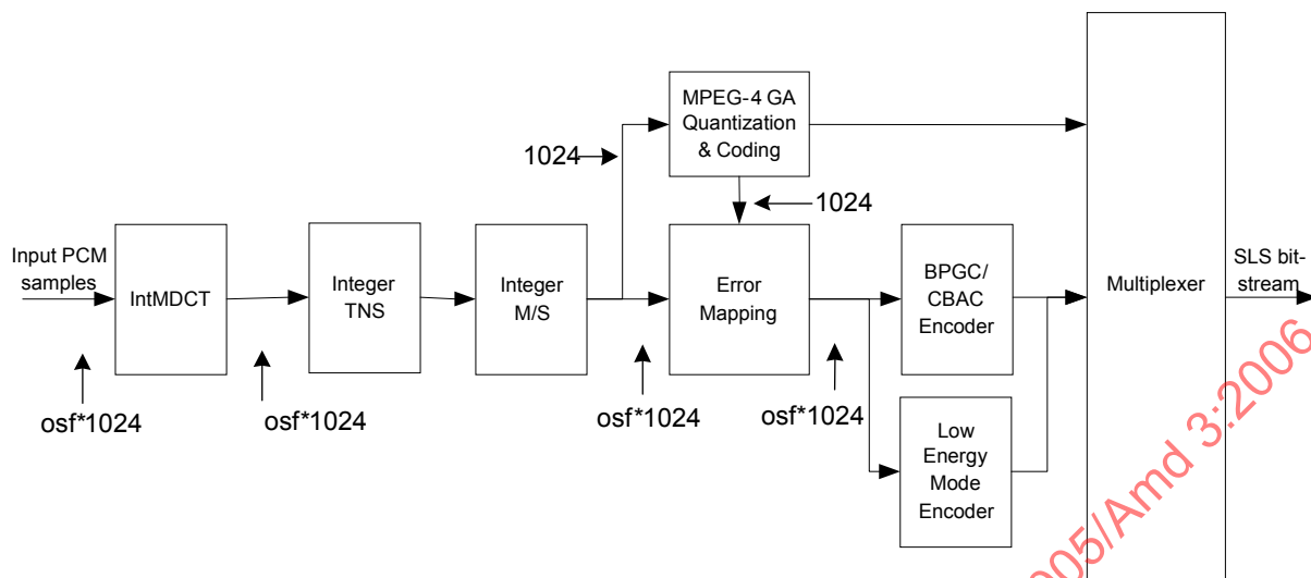
Figure 12.A.2 – Block diagram of SLS encoder with downsampling in the MDCT domain
