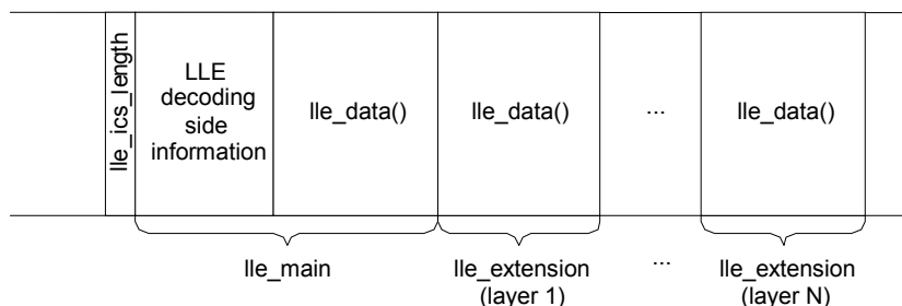
Figure 12.6 – Construction of LLE_ICS for from multiple LLE streams
