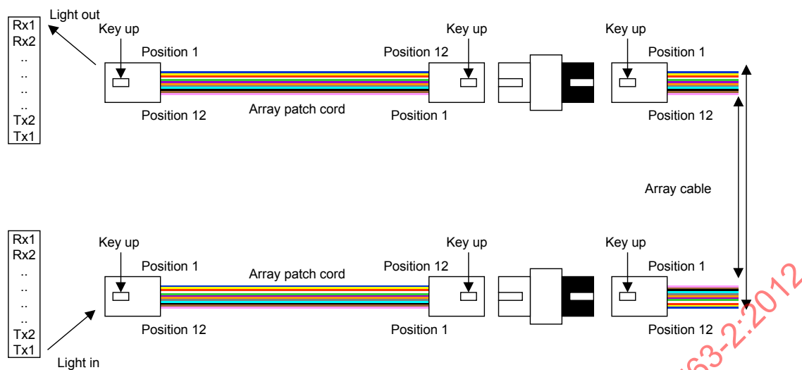
Figure A.11 – Connectivity method for parallel optics channels
