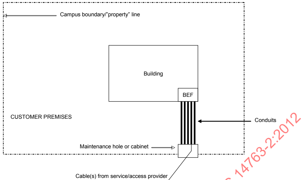
Figure B.2 – Example of a campus entrance facility
