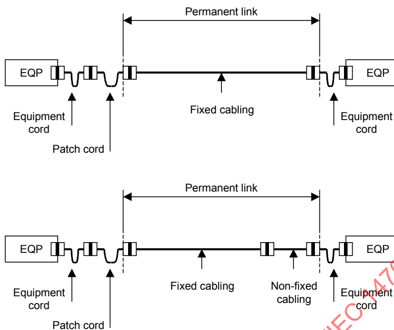
Figure 14 – Examples of cabling permanent links
