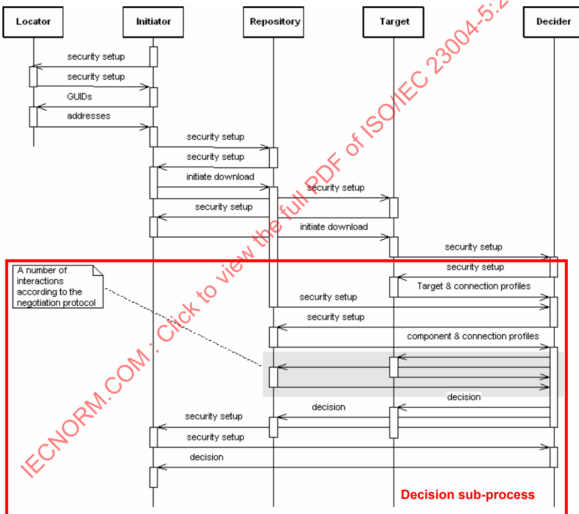
Figure 6 — Sequence diagram highlighting the decision sub-process
