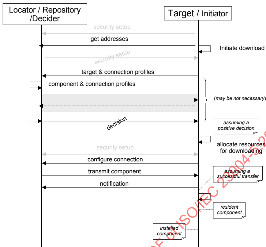
Figure A.4 — Sequence diagram initiator on target (single manufacturer)
