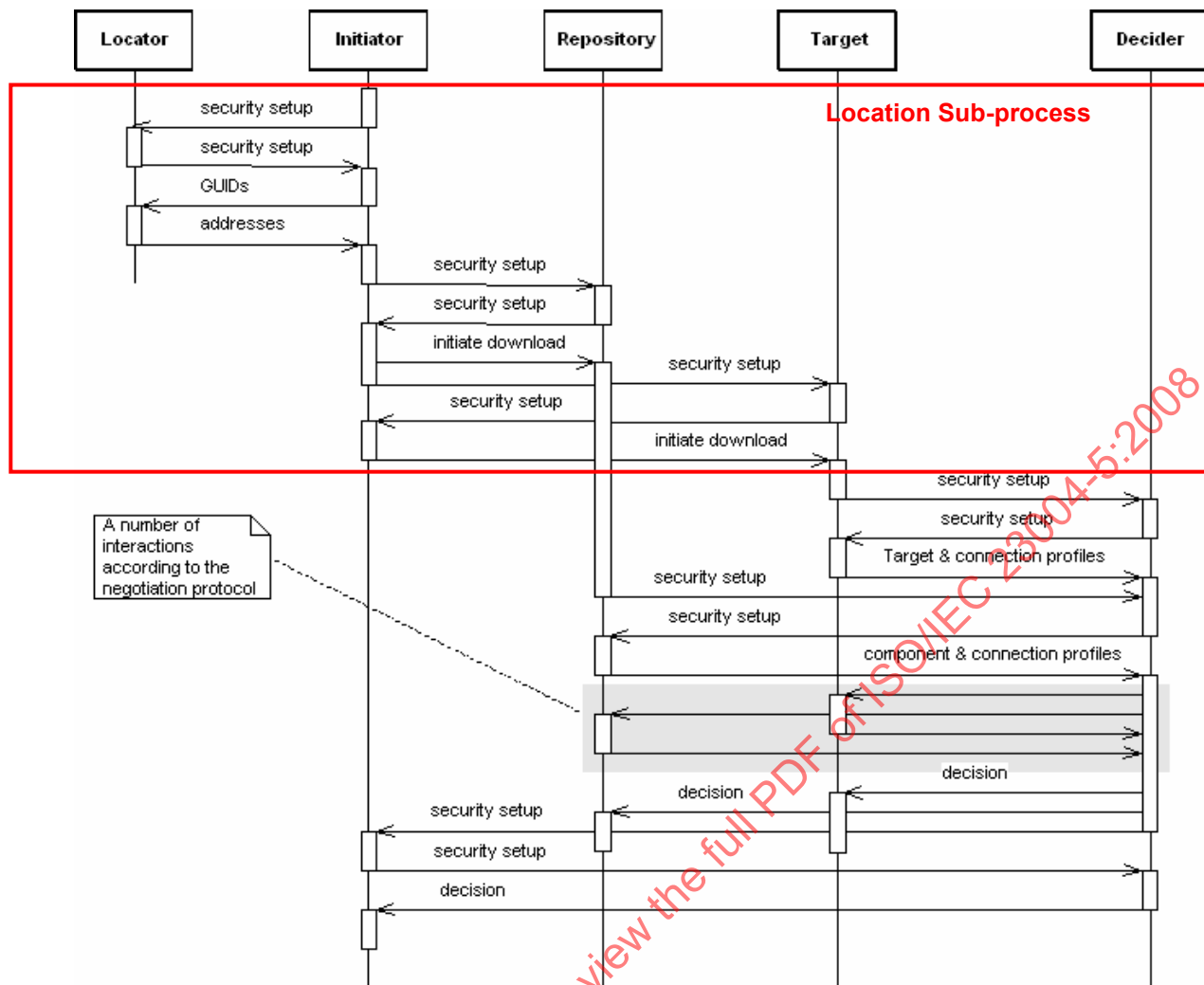
Figure 5 — Sequence diagram highlighting the location sub-process
