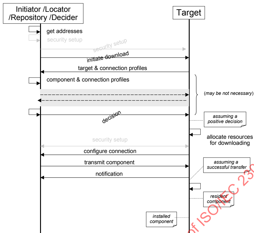
Figure A.2 — Sequence diagram initiator outside target
