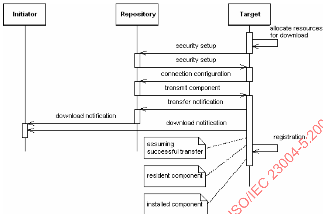
Figure 7 — Sequence diagram of Pull Transfer
