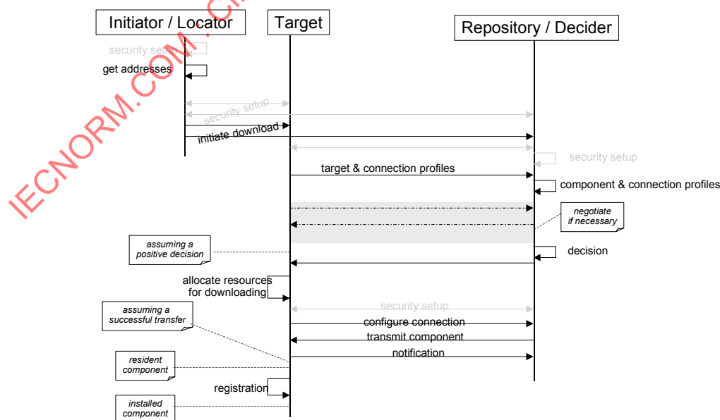
Figure A.8 — Sequence diagram initiator outside the target (multiple manufacturers)
