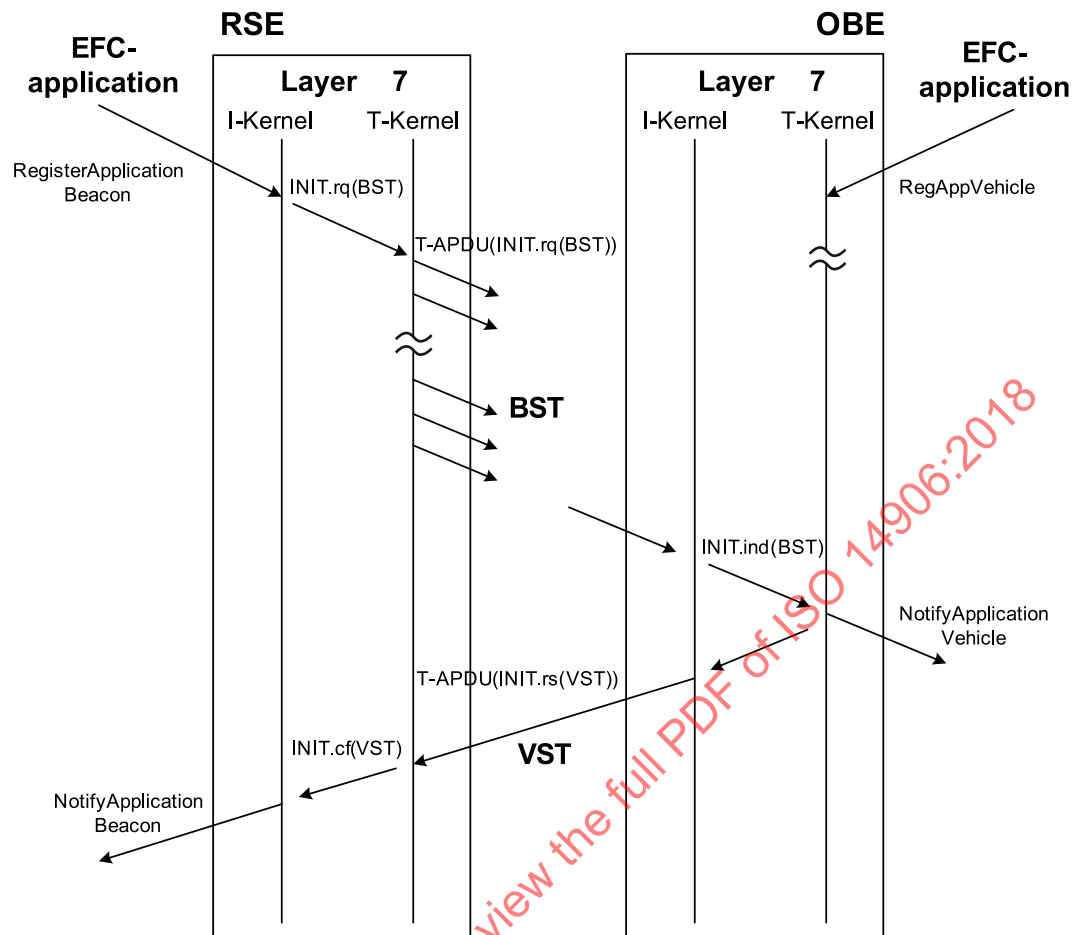
Figure 6 — Initialisation phase: BST - VST exchanges
