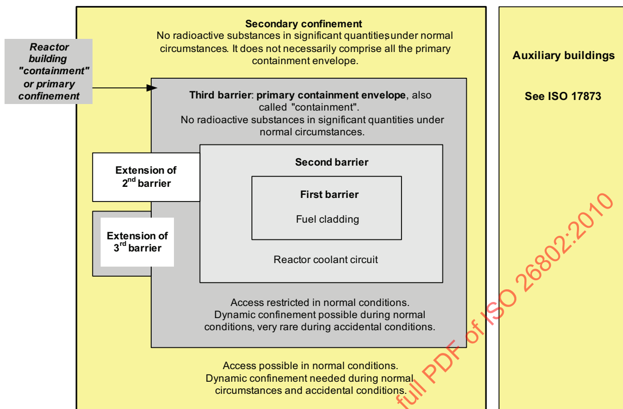
Figure 1 — Schematic diagram of reactor confinement systems
