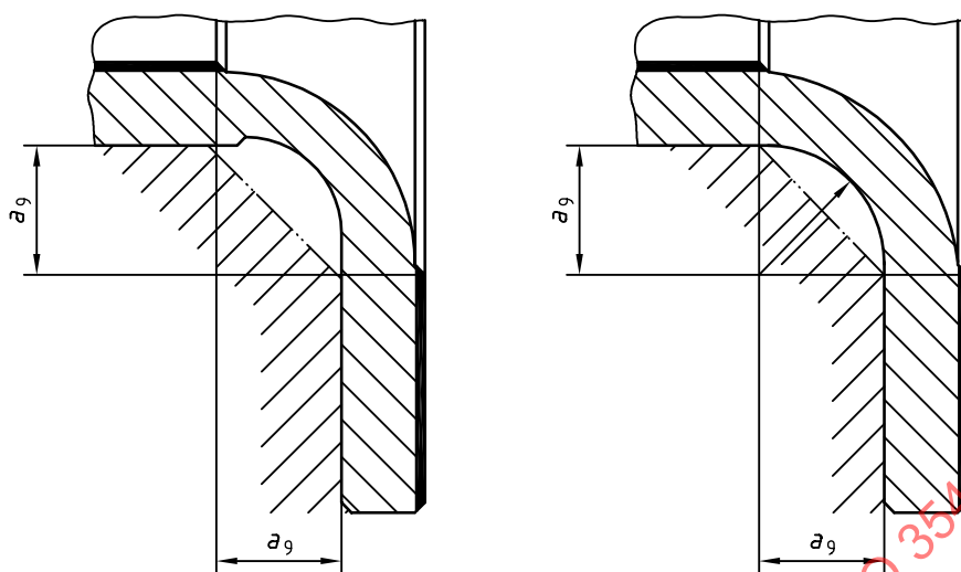
Figure 11 — Types of transition between radial parts of the flange
