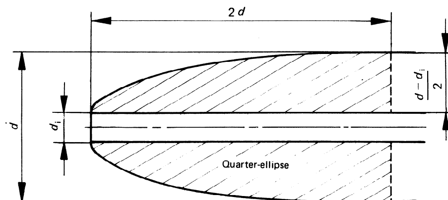
FIGURE 10 — Profile definition of the ellipsoidal head
