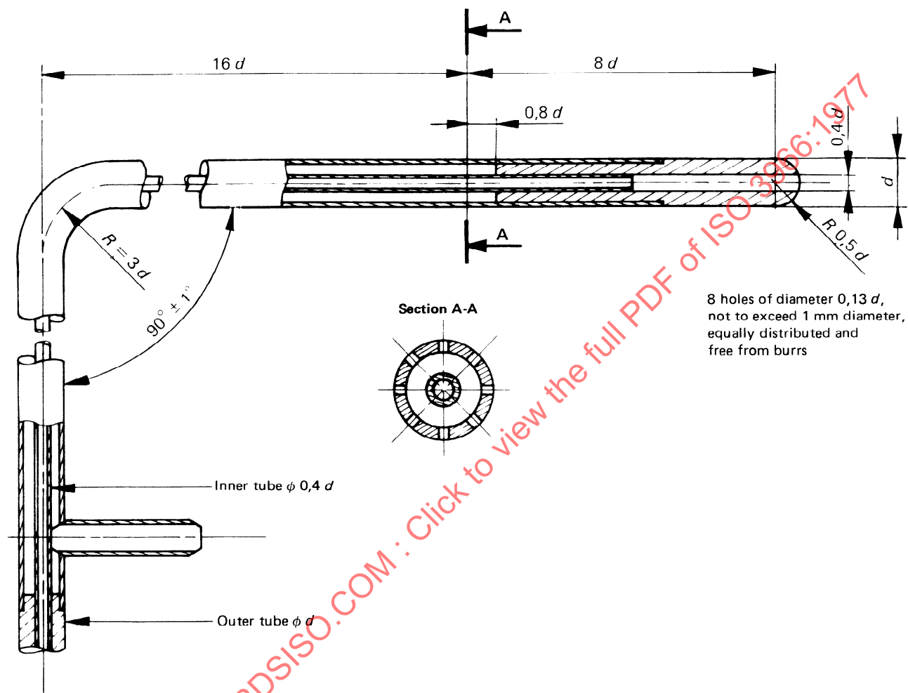
FIGURE 8 — AMCA type
