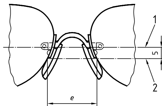
b) Rimless spectacle frame with pad bridge
