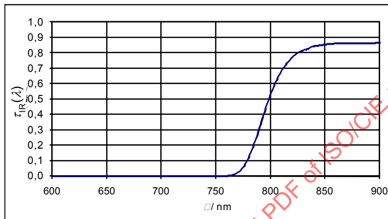
Figure 4 — Spectral transmittance \tau_{IR}(\lambda) of the IR filter for determination of the IR response f_{IR}
