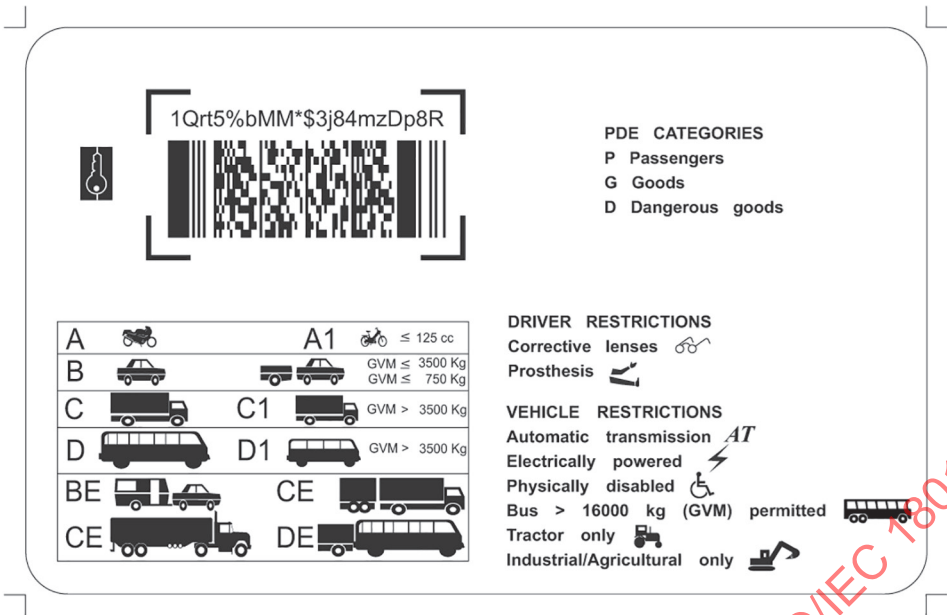
Figure A.14 — Informative example (not to scale)
