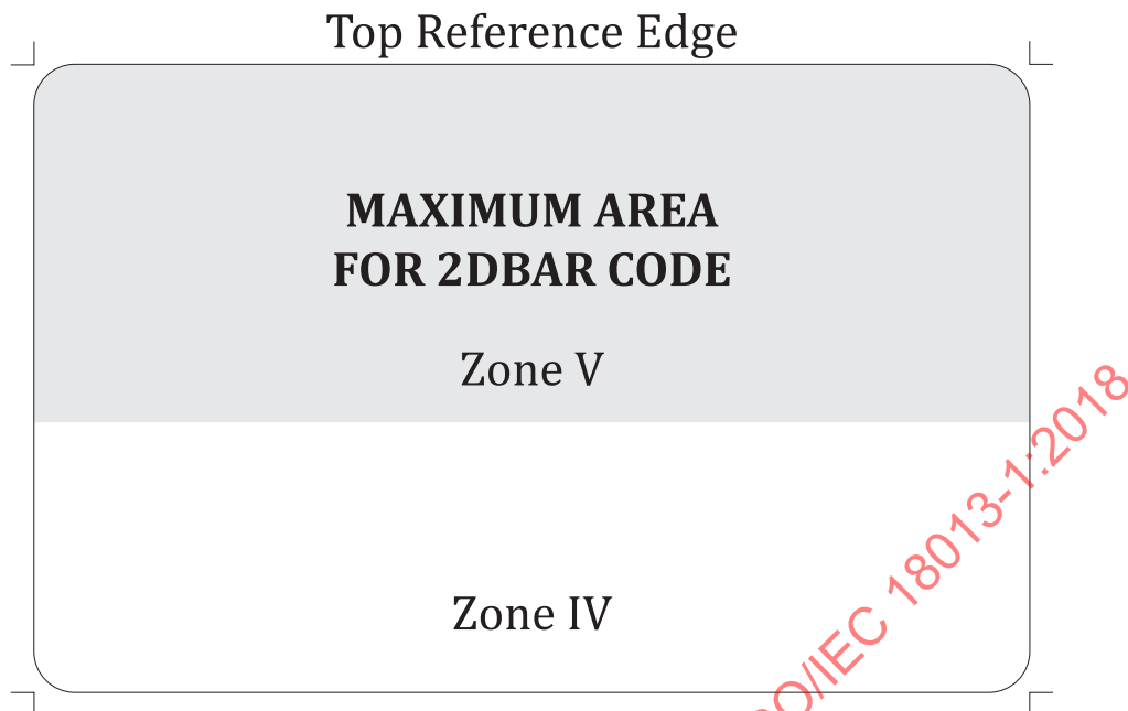
Figure A.12 — Non-portrait side of IDL — 2D bar code (not to scale)
