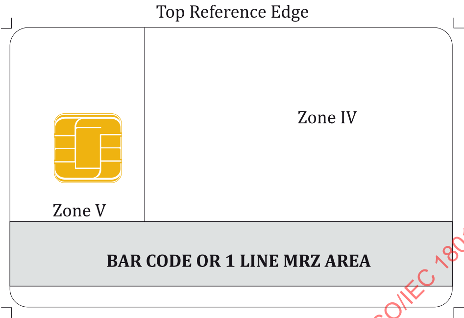
Figure A.18 — Non-portrait side of IDL – IC with contacts and bar code or 1 line MRZ (not to scale)
