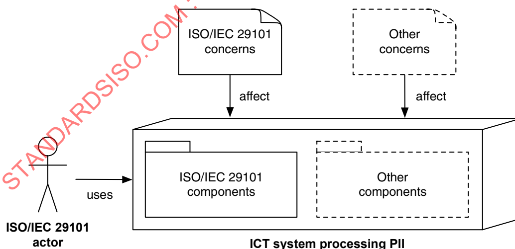
Figure 1 — Elements of the privacy architecture framework in context
