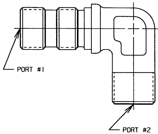
FIGURE 2 - FITTING, ELBOW, 90 DEGREE, BULKHEAD END FOR OPTIONAL USE IN PORT INSTALLATION, SHOWN AS NON-REDUCER, SAME AS FIGURE 1 EXCEPT AS SHOWN
