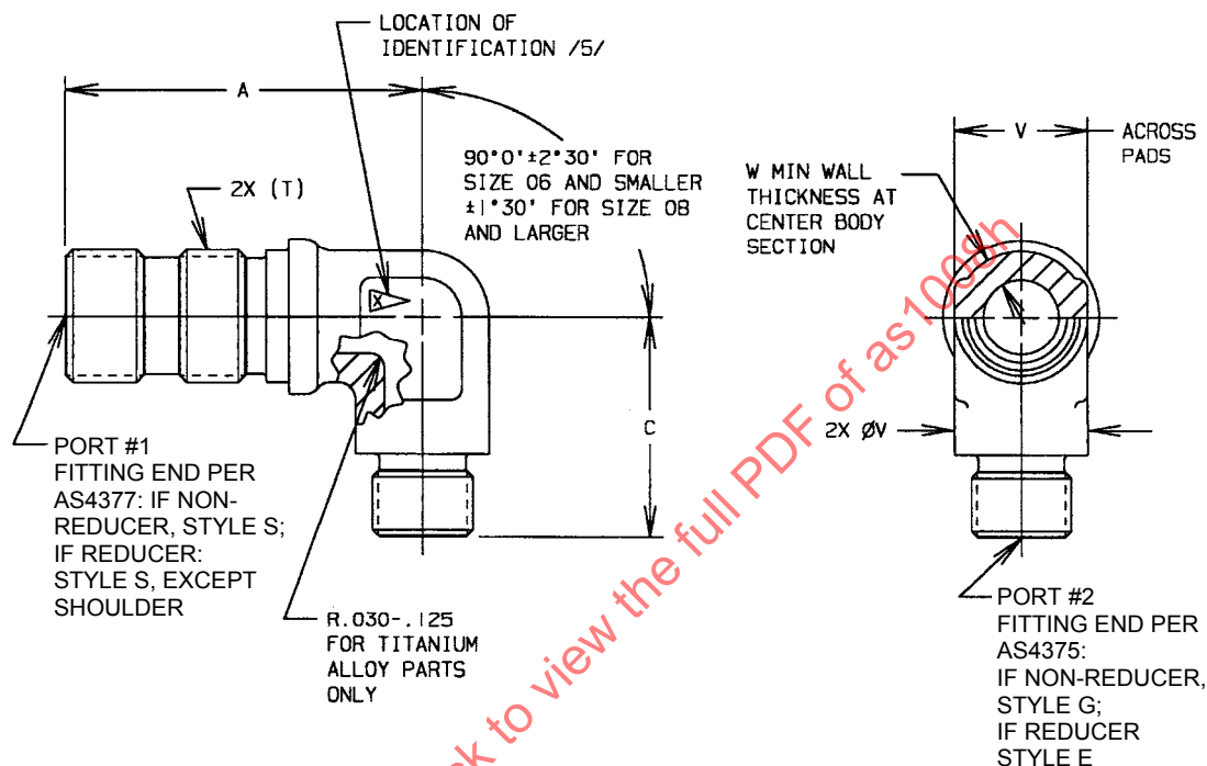
FIGURE 1 - FITTING, ELBOW, 90°, BULKHEAD END FOR OPTIONAL USE IN PORT INSTALLATION, PORT #2 SHOWN AS REDUCER
