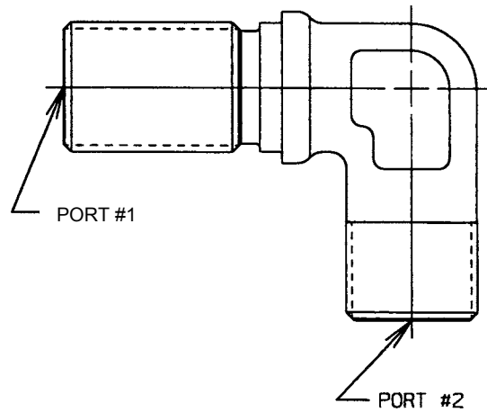
FIGURE 4 - FITTING, ELBOW, 90 DEGREE, BULKHEAD END NOT FOR USE IN PORT INSTALLATION, SHOWN AS NON-REDUCER, SAME AS FIGURE 2 EXCEPT AS SHOWN
