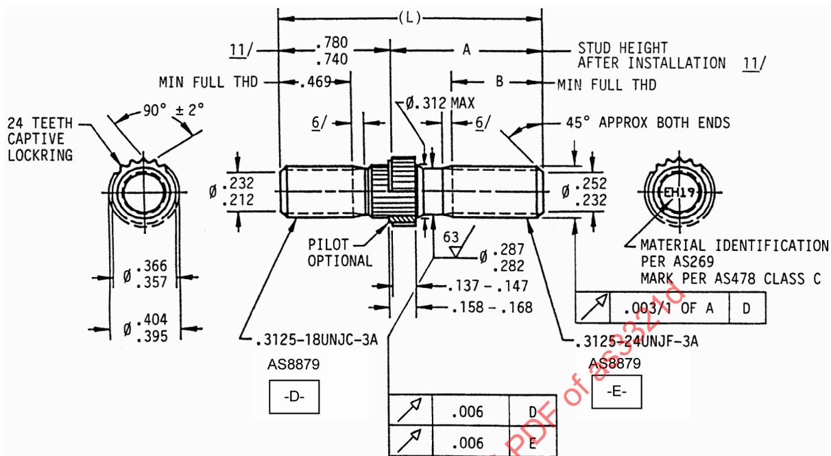
FIGURE 1 - STUD
