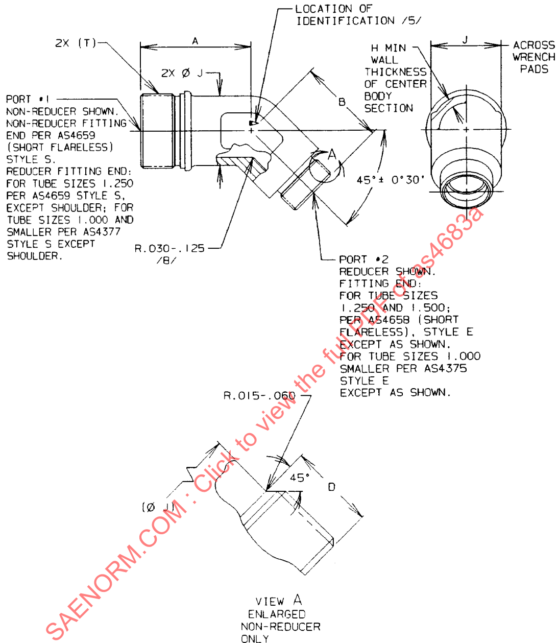
FIGURE 1 - FITTING, ELBOW, 45°, REDUCER
