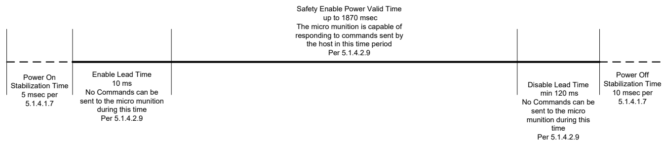
FIGURE 8 – SAFETY ENABLE POWER TIMELINE
