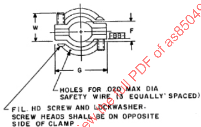
FIGURE 2 - DIMENSIONS AND CONFIGURATIONS (NON-SELF-LOCKING ONLY)
