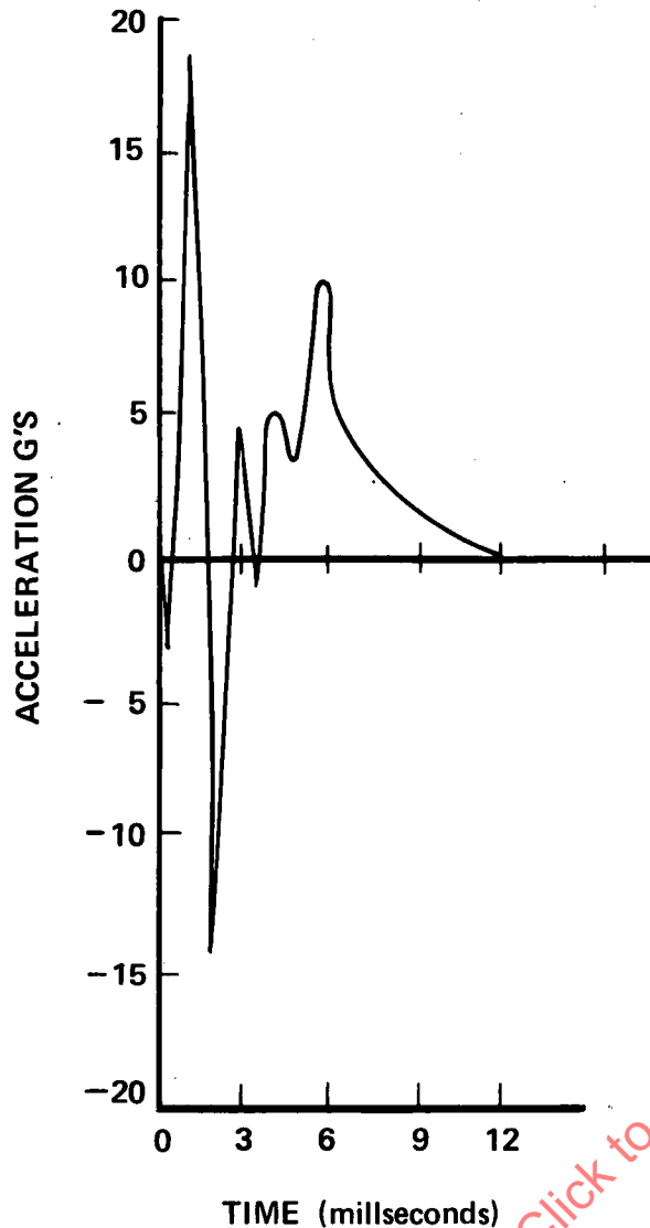
FIG. 5—OPERATIONAL SHOCK PROFILE
