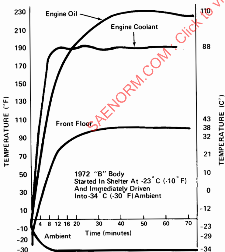
FIG. 1—VEHICLE COLD WEATHER WARM-UP CHARACTERISTICS
