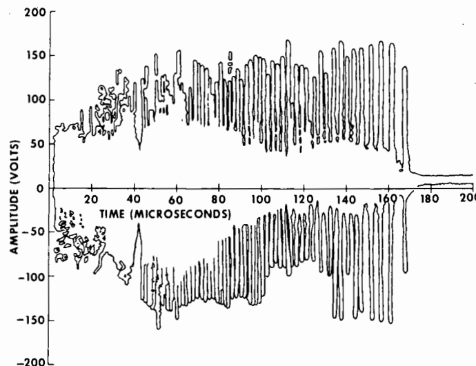
FIG. 9—POWER LINE ELECTRICAL NOISE
