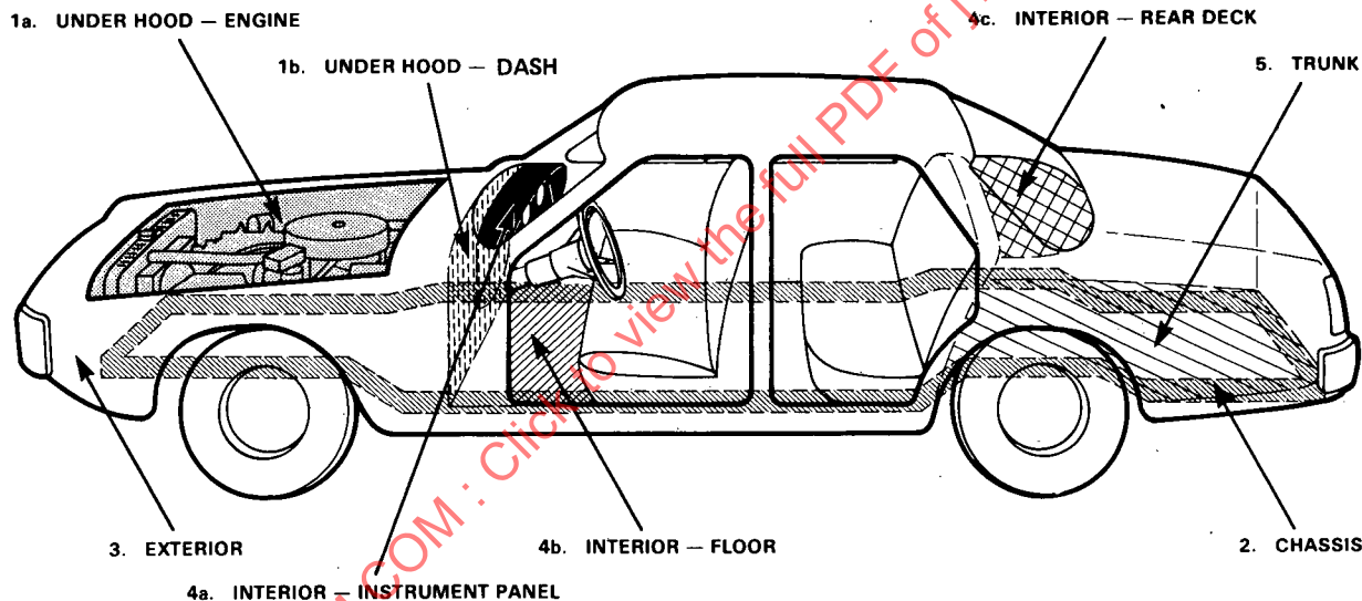
FIG. 10—VEHICLE ENVIRONMENTAL ZONES
