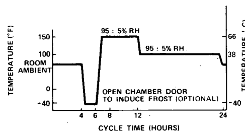
FIG. 3A-24-H CYCLE
