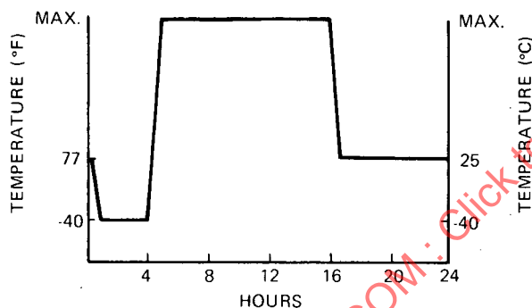
FIG. 2A-24-H CYCLE
