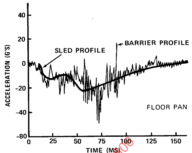
FIG. 6—48 KM/H (30 MPH) BARRIER AND SLED SHOCK PROFILES
