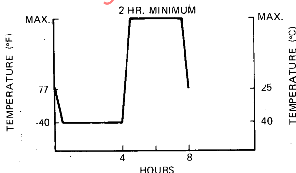
FIG. 2B-8-H CYCLE
