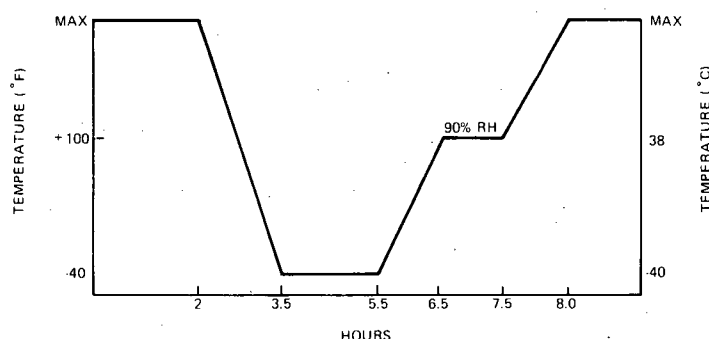
FIG. 3B-8-H CYCLE
