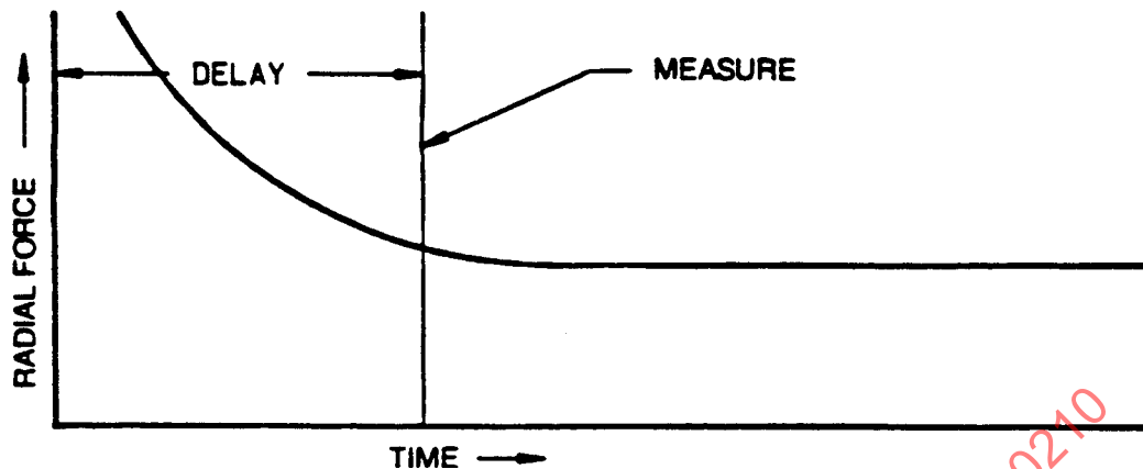
FIGURE 3—STRESS RELAXATION CURVE
