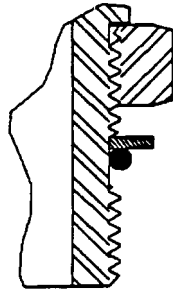
FIGURE B1—LOCKNUT BACKED OFF
