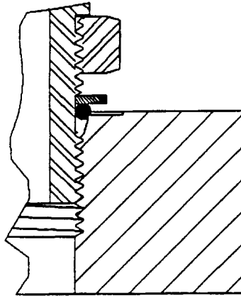
FIGURE B3—FITTING BACKED-OFF FOR ALIGNMENT (1 TURN MAXIMUM)
