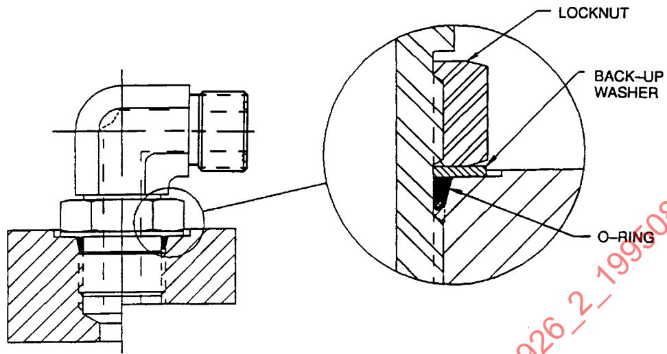
FIGURE B5—FINAL ASSEMBLY OF ADJUSTABLE STUD END
