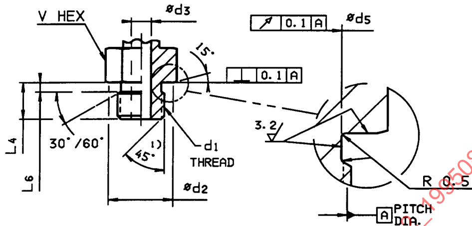
FIGURE 1B—NONADJUSTABLE SAE J1926/2 HEAVY-DUTY (S SERIES) STUD END DETAIL
