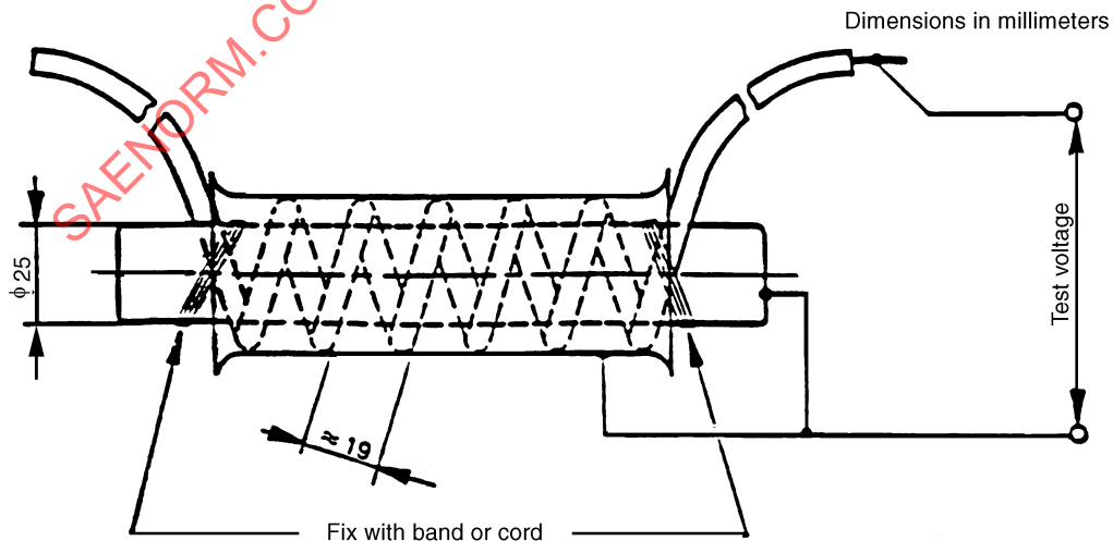
FIGURE A2—TEST APPARATUS FOR CORONA RESISTANCE TEST
