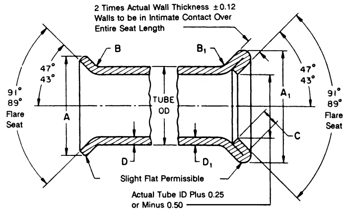
FIGURE 1—SINGLE AND DOUBLE 45-DEGREE FLARES FOR TUBING
