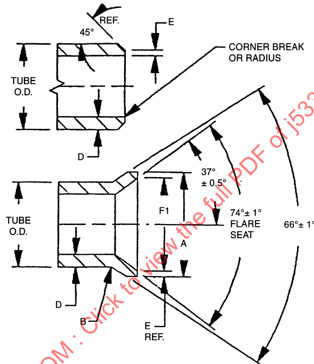
FIGURE 3—OPTIONAL TUBE PREPARATION AND SINGLE 37-DEGREE FLARE FOR TUBING
