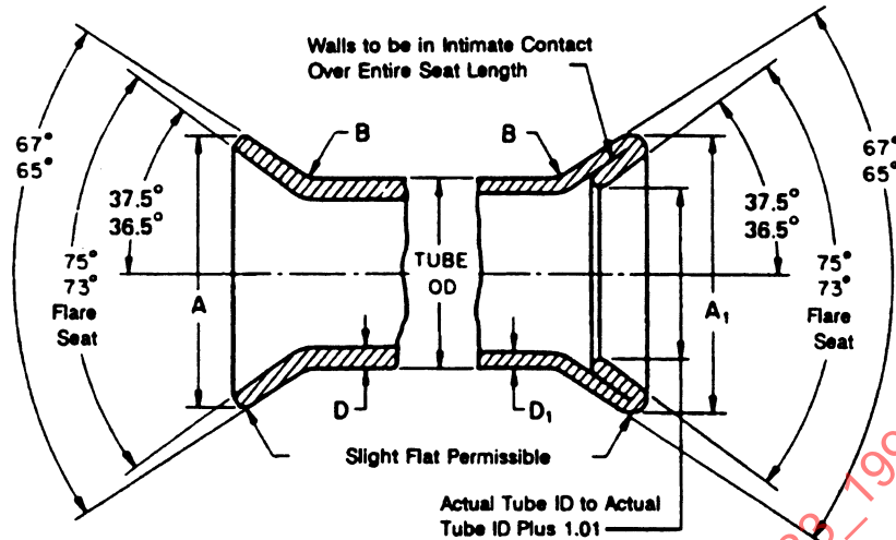
FIGURE 2—SINGLE AND DOUBLE 37-DEGREE FLARES FOR TUBING
