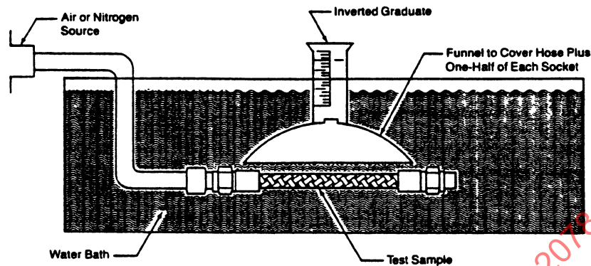
FIGURE 3 - Test Setup for Pneumatic Effusion Tests
