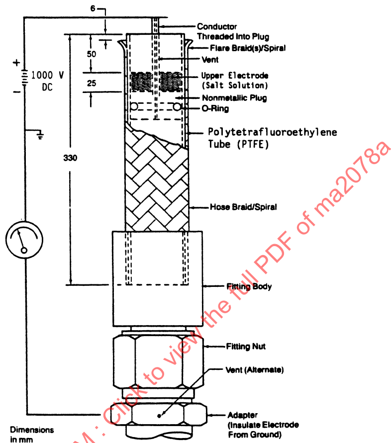
FIGURE 4 - Conductivity Test Setup, Braided Hose
