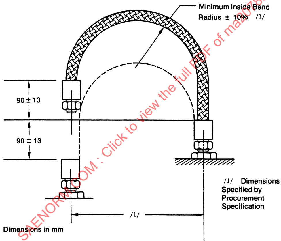
FIGURE 6 - Flexure Test Setup
