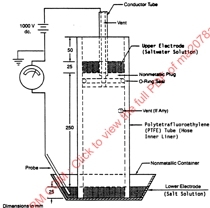
FIGURE 2 - Diagram for the Electrical Conductivity Test of Lining
